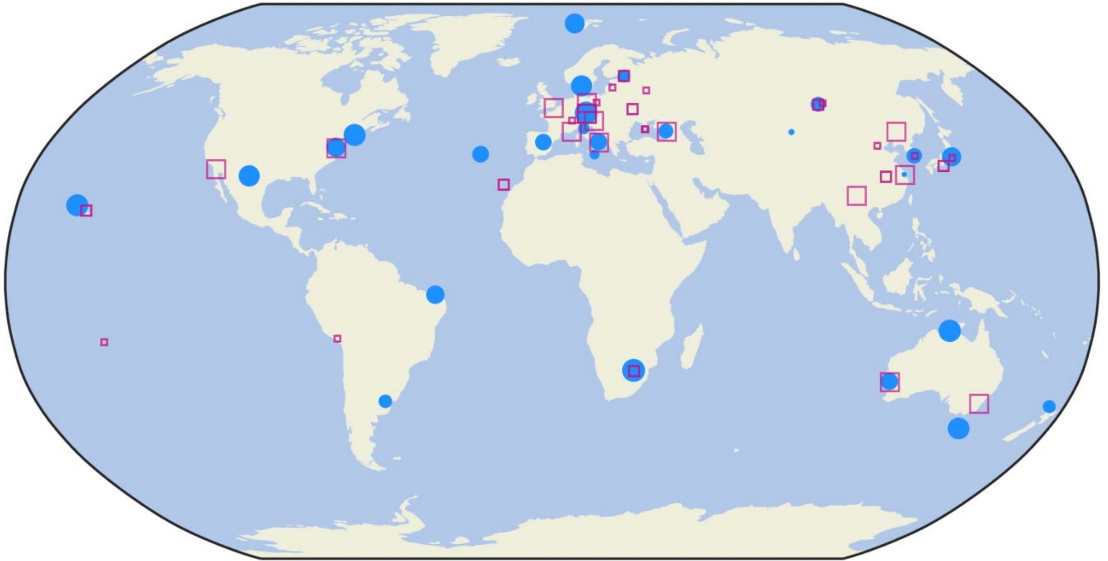
Figure: Locations of ground-based VLBI stations and SLR stations. The size of the circles and squares are roughly proportional to how much data each station provides to the global geodesy supply chain. The data is from 2023-2024.
